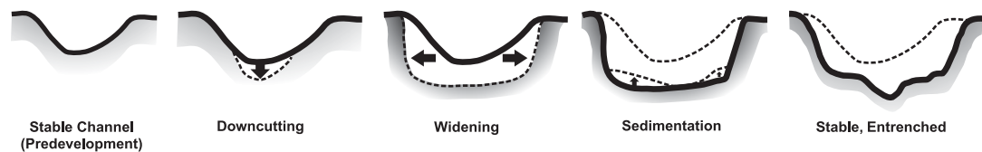
Figure 1-6 Changes to a Stream's Physical Character Due to Urban Development
