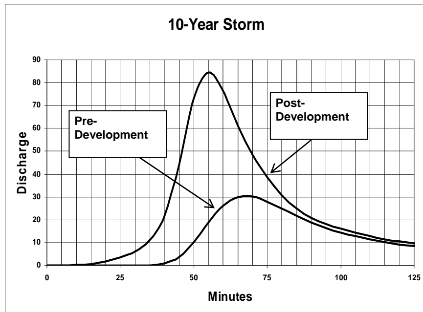
Figure 1-5 Hydrograph under Pre- and Post Development Conditions
