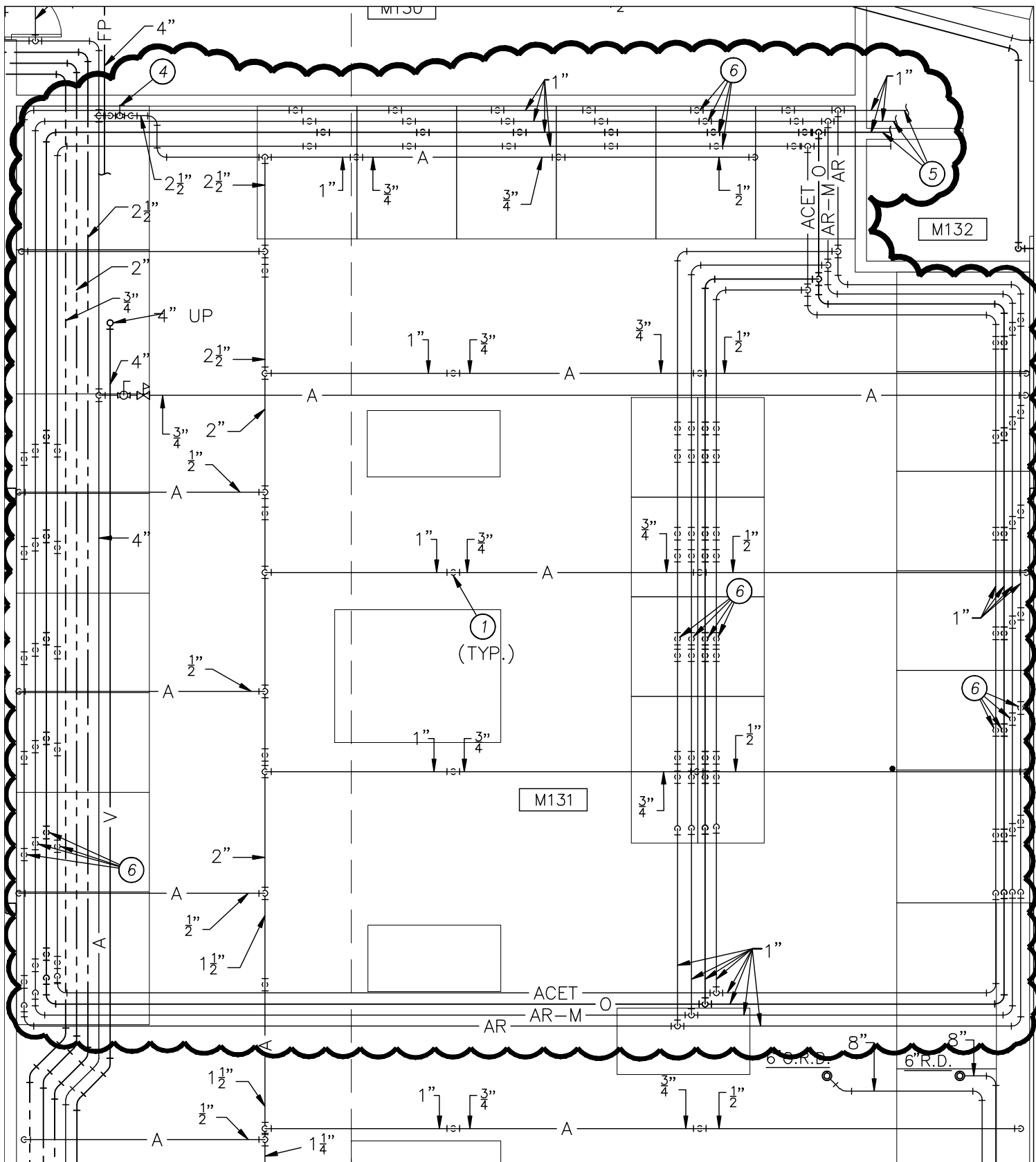
PARTIAL M3.17 PLAN SCALE: 1/8" = 1'-0"
