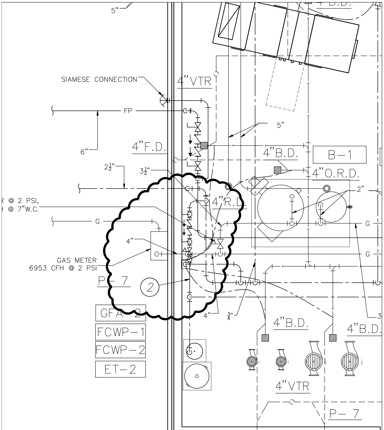
PARTIAL M3.17 PLAN SCALE: 1/4" = 1'-0"
