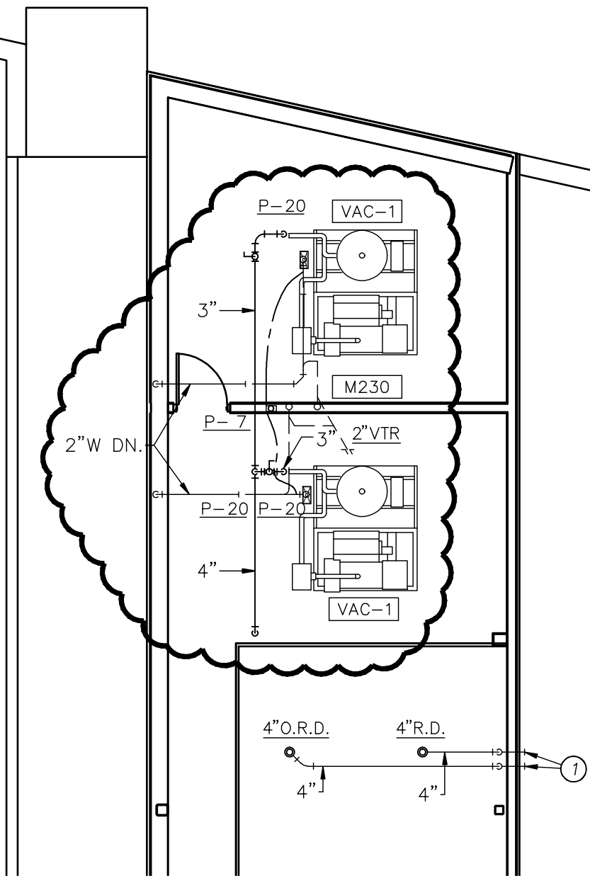
PARTIAL M3.26 PLAN SCALE: 1/8" = 1'-0"
